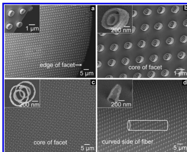
Figure 4. (a) A portion of an optical fiber bearing an array of concentric gold rings. (b) The core of the same optical fiber as shown in (a). The structures have 50 nm thick walls, and are 400 nm tall. (c) The core of an optical fiber bearing overlapping arrays of concentric gold rings. (d) An array of gold split cylinders on the curved (cylindrical) side of a stripped optical fiber. The long axis of the optical fiber is parallel to the long axis of the outline drawing of the cylinder.
