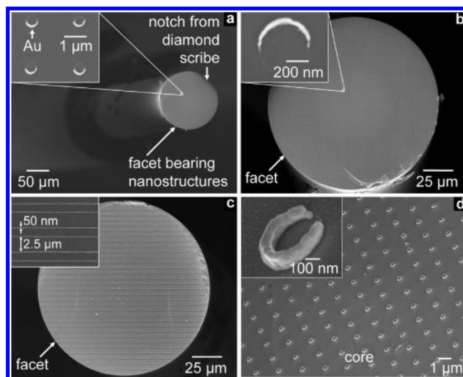
Figure 3. (a) An optical fiber bearing an array of gold crescents (shown in the inset). (b) A close-up of the facet. The inset is a single gold crescent. (c) A facet bearing a grating of gold nanowires. (d) The core of a fiber bearing an array of gold split rings.
