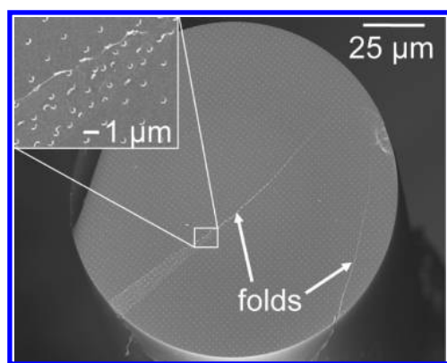
Figure 5. A facet bearing a poorly transferred array of crescents. There was a fold in the epoxy slab as it was transferred to the fiber. The inset shows a region of the fold, which contains jumbled nanostructures.
