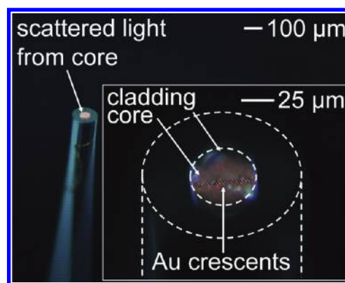
Figure 6. Optical image of a cleaved facet of an optical fiber supporting an array of gold crescents. Light from a halogen source is coupled to the core of the fiber at the opposite end of the fiber. The inset is a close-up of the facet. Light, supplied by the fiber, scatters from the gold nanostructures on the core of the optical fiber and not those on the cladding. The fiber is tilted \sim 45^\circ to isolate only the light scattered from the nanostructures (tilting prevents nonscattered light from the fiber from entering the objective of the microscope directly).
