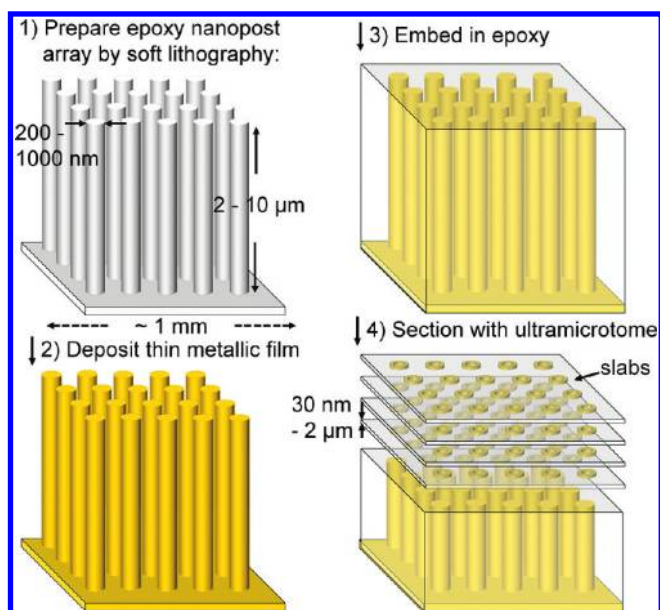
Figure 1. Example of a procedure used to fabricate arrays of metallic nanostructures by embedding and sectioning a metallized array of epoxy nanoposts using an ultramicrotome. This procedure produces manipulable slabs of epoxy containing arrays of metallic nanostructures.
