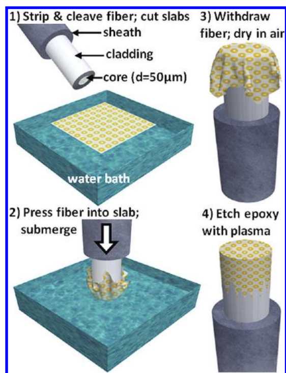
Figure 2. Summary of the procedure used to fabricate and transfer arrays of metallic nanostructures to the facets of optical fibers.
