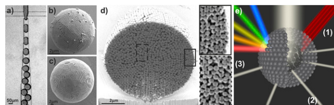
Fig. 1. Photonic balls are prepared by self-assembly of colloids in the spherical confinement of emulsion droplets. ( A ) Optical micrograph of the cross-junction microfluidic device used to emulsify a colloidal dispersion into monodisperse droplets. ( B and C ) SEM micrographs of photonic balls formed by assembly of 250-nm colloids in the confinement of an emulsion droplet ( d_{\text{ball}} = 8 \mu\text{m} in B and 30 \mu\text{m} in C ). Moiré patterns visible in C indicate high order. ( D ) Exemplary cross section of a photonic ball obtained by FIB cutting indicates a layered internal morphology with ordered structure around the interface ( Top Inset ) and increasing disorder toward the center ( Bottom Inset ). See Fig. S2 for further examples. ( E ) Schematic illustration of multiple optical effects originating from the hierarchical self-assembly (1): Crystalline order results in Bragg reflection of light with a wavelength defined by the colloid size (2); disorder in the assembly gives rise to unselective scattering of incident light (3); periodic assemblies at the ball's surface lead to grating diffraction effects, separating white light into its spectral components (for colloid sizes > 400 nm).
