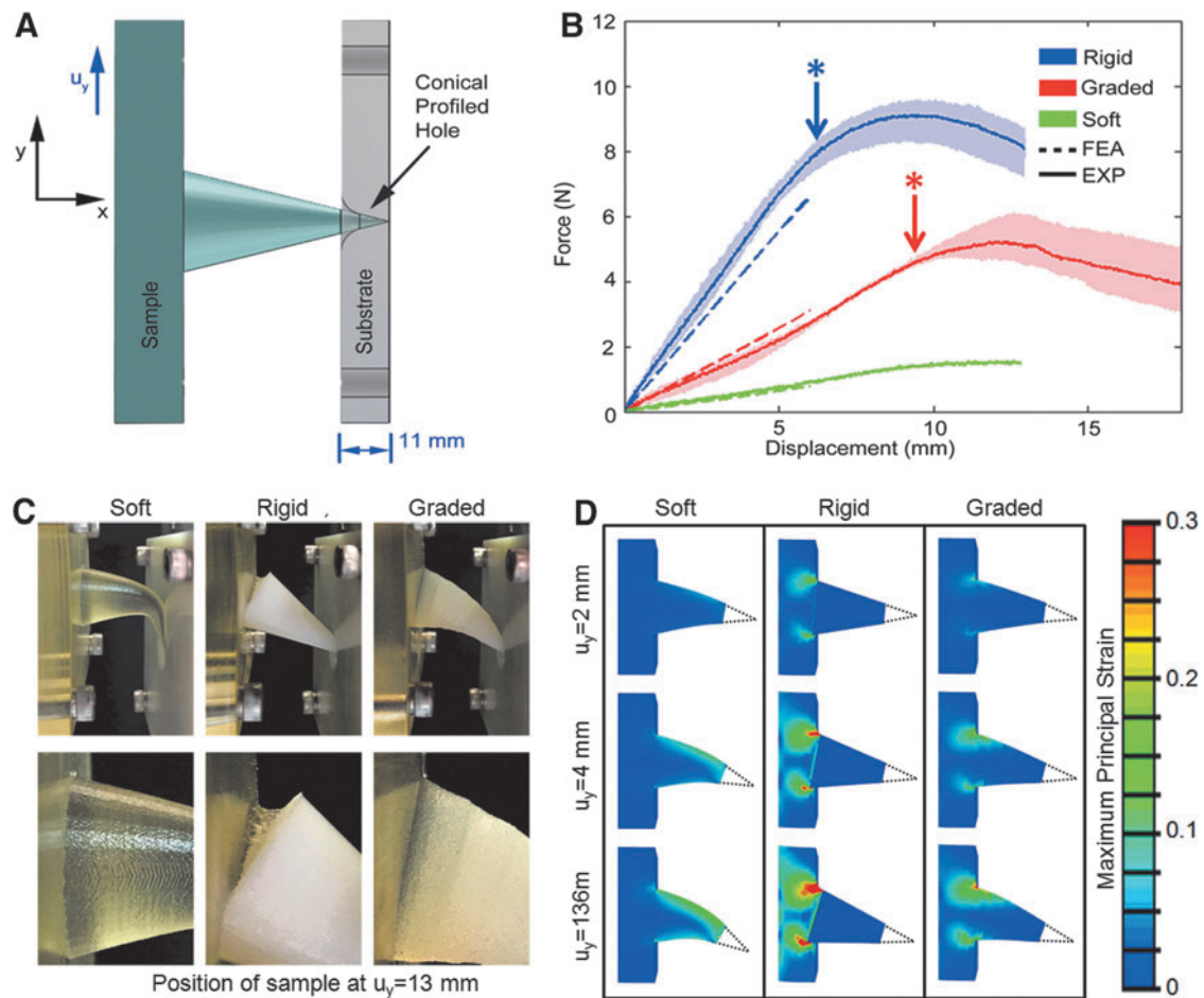
FIG. 3. Experimental and simulated shear tests of soft, rigid, and functionally graded conical tooth-like elements attached to a flexible base. We simultaneously measured the flexibility and anchoring of the three conical designs inside the punctured object under shear stress, while monitoring the integrity of the interface between the cone and its flexible substrate. (A) Schematic illustration of the shear testing rig. The conical sample was clamped 11 mm below the tip inside a 3D-printed conical profiled reference hole in the substrate and was displaced in the y -axis relative to the substrate. (B) Experimental (solid lines) and simulated (dashed lines) force displacement plots for the fully rigid, functionally graded, and soft conical configurations. The shaded region around each plot represents the standard deviation ( n=4 ) for each model. The blue asterisk indicates the point of interfacial failure in the rigid cone, and the red asterisk indicates the load at which the functionally graded cone displacement is transferred to the flexible base. (C) Photographs of the three conical models at displacement u_y = 13 mm (i.e., failure point for rigid and soft conical models) show the global cone deformation (top images) and the effect of shear force on the interface adjoining cones and the soft substrates (bottom images). The tip of the soft cone is dislodged from the reference hole and shows the worst anchoring stability inside the punctured reference object, whereas the rigid sample shows the maximum interfacial damage among the three conical models. (D) Simulated maximum principal strain distribution within the samples at shear displacements of u_y = 2, 4, and 6 mm.
