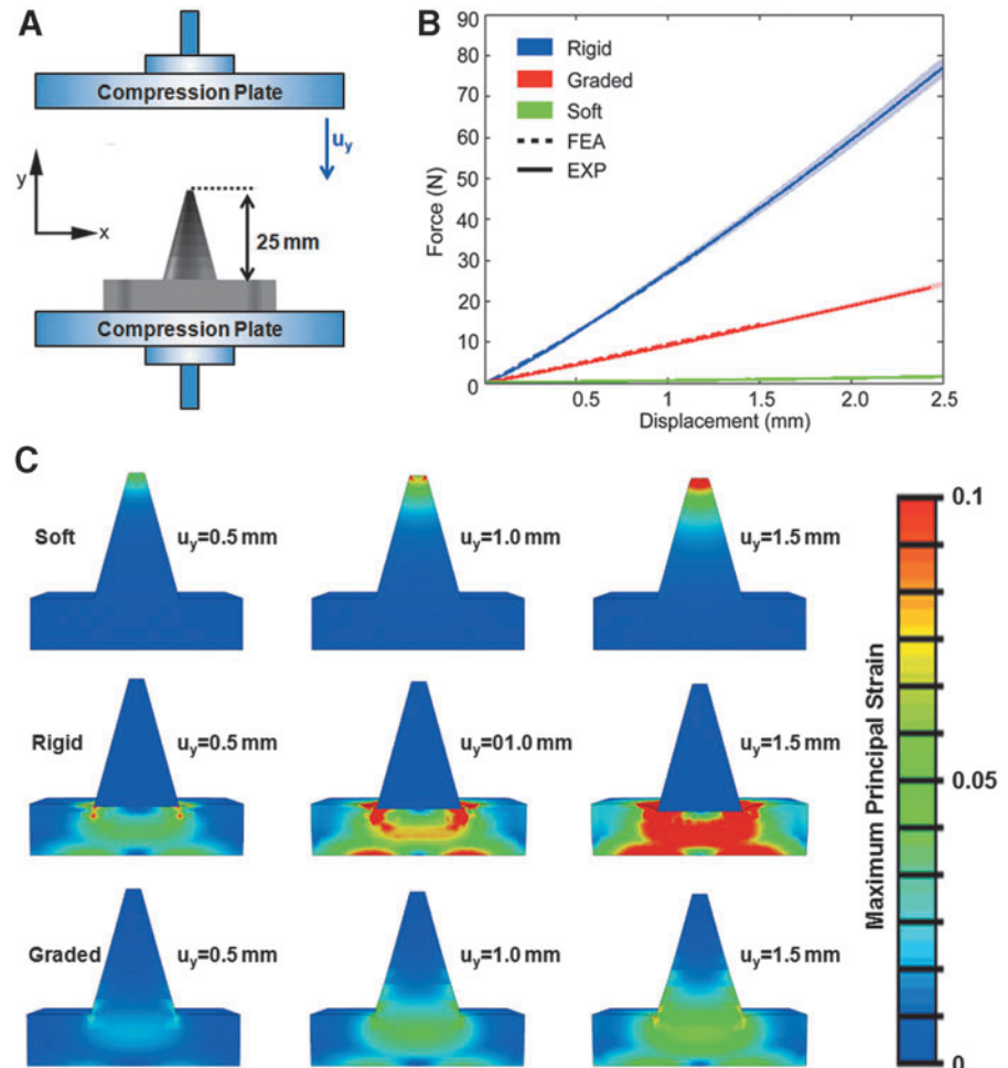
FIG. 4. Experimental and simulated compression tests of soft, rigid, and functionally graded conical tooth-like elements attached to a flexible base. (A) Schematic illustration of the compression testing rig. The conical sample, truncated at 5 mm below the tip, was compressed between two parallel plates by applying displacement u_y along the y -axis. (B) Experimental (solid lines) and simulated (dashed lines) compression response of fully rigid, graded, and soft conical models. The shaded region around each plot represents the standard deviation ( n=4 ) for each model. (C) Simulated maximum principal strain distribution within the samples at displacements of u_y = 0.5, 1.0, \text{ and } 1.5 \text{ mm} .
